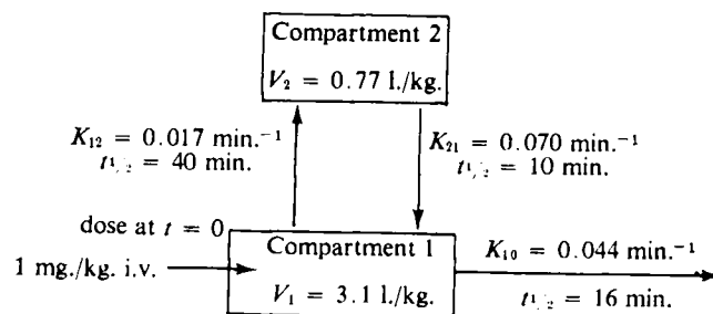
Scheme 1—Two-compartment open pharmacokinetic model for intravenous naloxone
