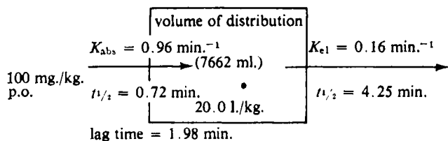
Scheme II—One-compartment open model for orally administered naloxone
